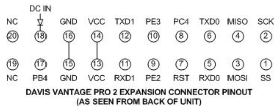
Figure 5: The Davis Vantage Pro2 rear expansion connector, as described by DeKay [10]. NOTE: Pin numbers/orientation as seen when looking directly at the exposed connector at the rear of the console.
