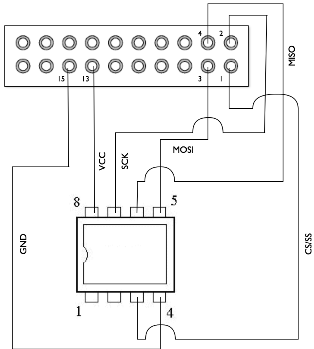
Figure 18: Required wiring between the console expansion connector and the MCU. Refer to figure 5 for a description of the expansion connector.
