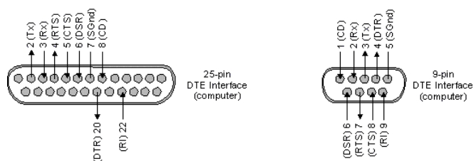
Figure 20: Data Terminal Equipment (DTE) pin numbering for the 25-pin and 9-pin connectors normally used for serial-line communications. In other words, the above pin numbers appear "as seen" when looking directly at a PC-side COM port.
